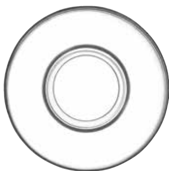
eda eda269 tea saucer, h: 18 mm, 2/3 in, Ø: 115 mm
